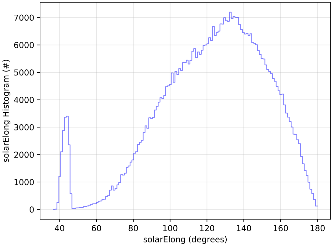
too_elab_r32_d3_griz_v3.4_10yrs WFD r band: solarElong Histogram
