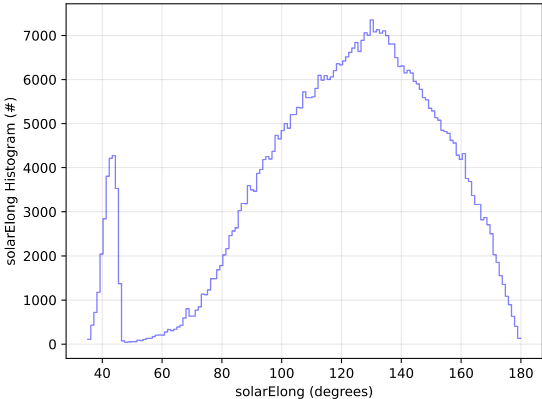
too_elab_r32_d3_griz_v3.4_10yrs WFD i band: solarElong Histogram
