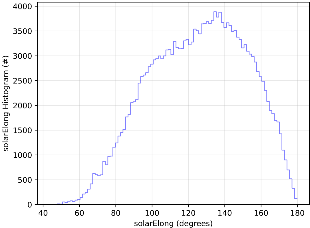
too_elab_r32_d3_griz_v3.4_10yrs WFD g band: solarElong Histogram
