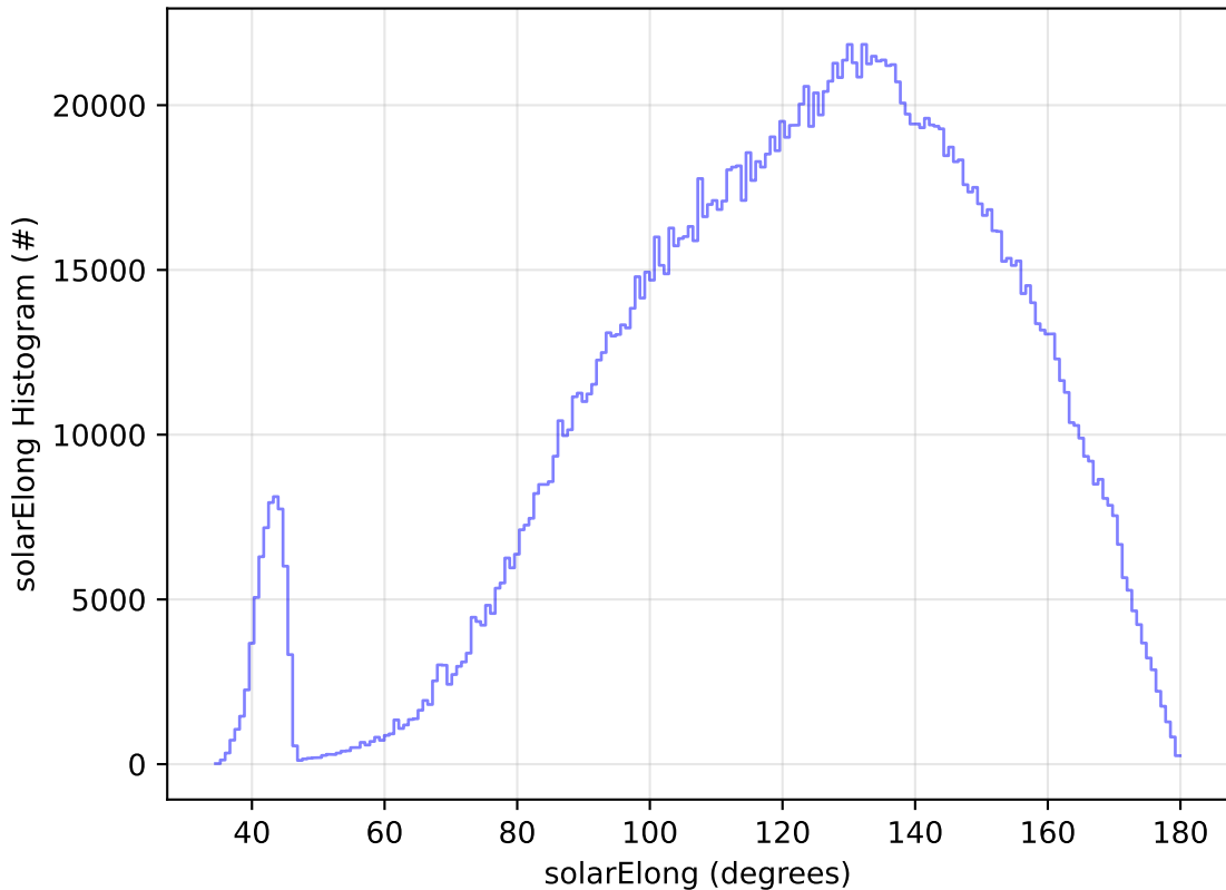
too_elab_r32_d3_griz_v3.4_10yrs WFD all bands: solarElong Histogram
