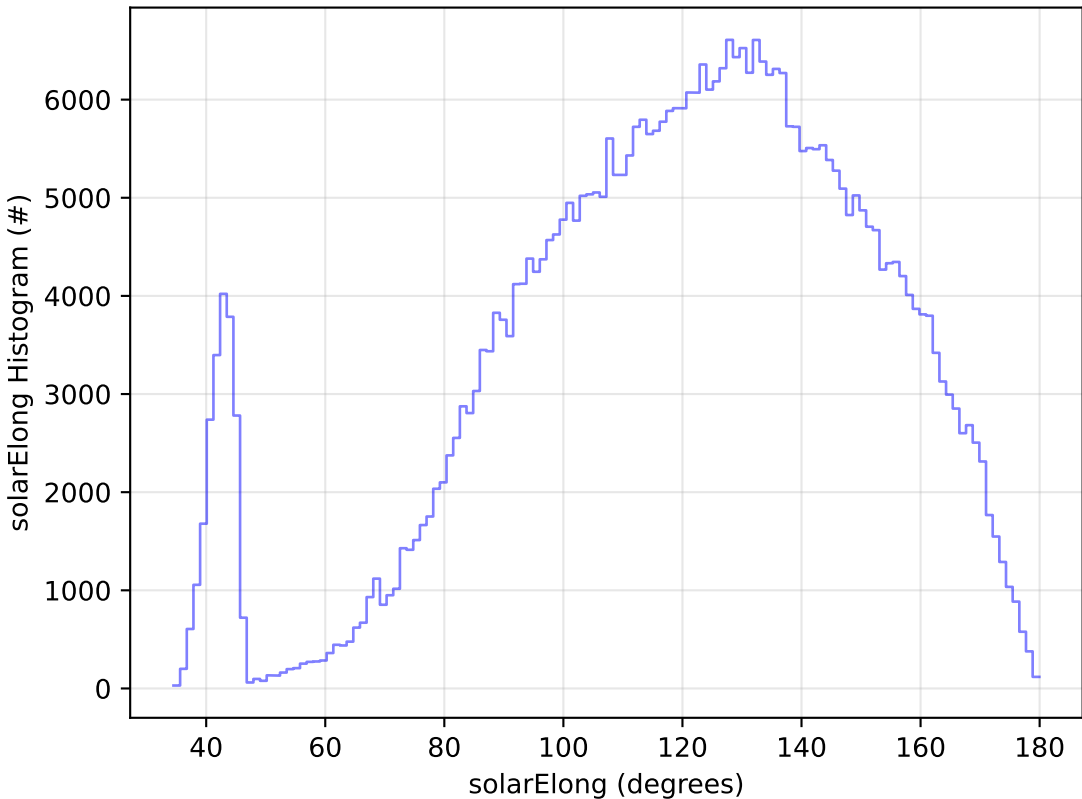
too_elab_r32_d3_griz_v3.4_10yrs All sky z band: solarElong Histogram
