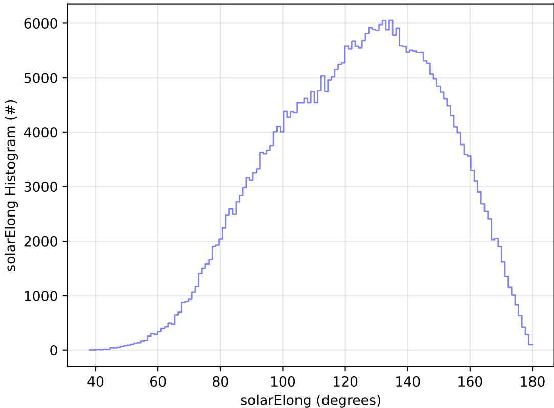
too_elab_r32_d3_griz_v3.4_10yrs All sky y band: solarElong Histogram
