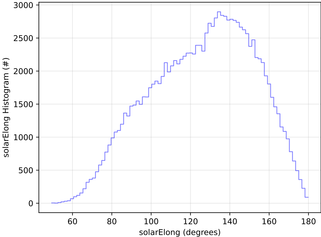
too_elab_r32_d3_griz_v3.4_10yrs All sky u band: solarElong Histogram
