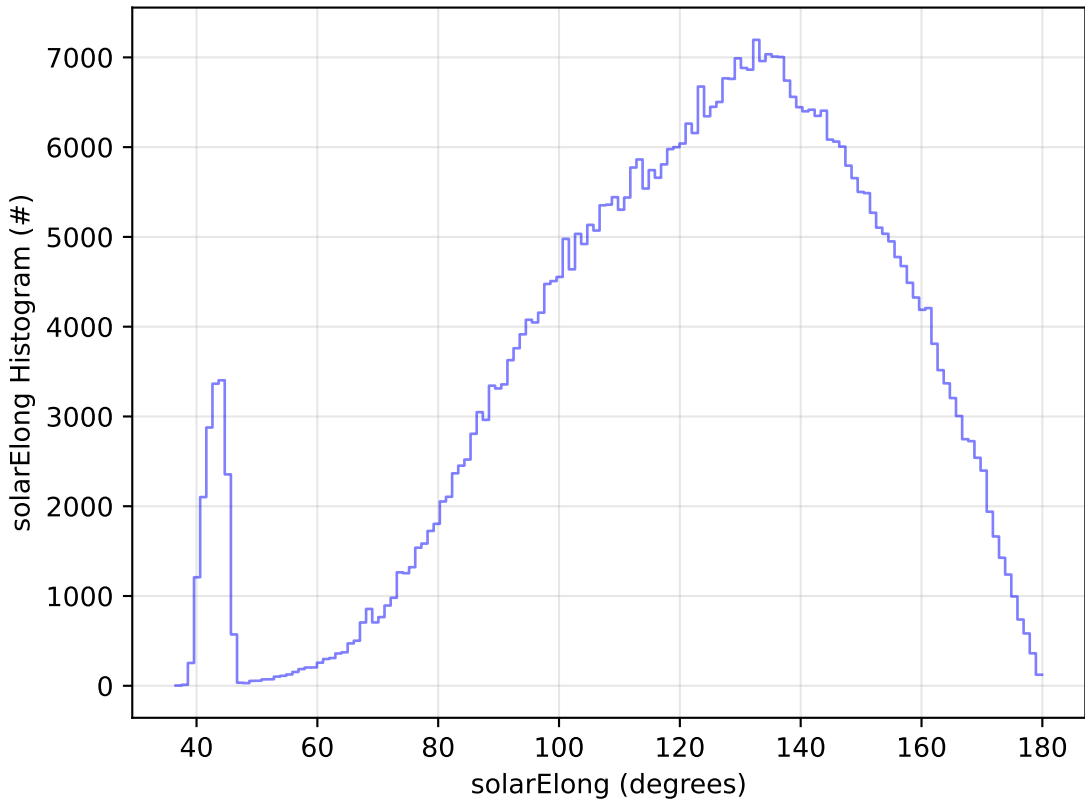
too_elab_r32_d3_griz_v3.4_10yrs All sky r band: solarElong Histogram
