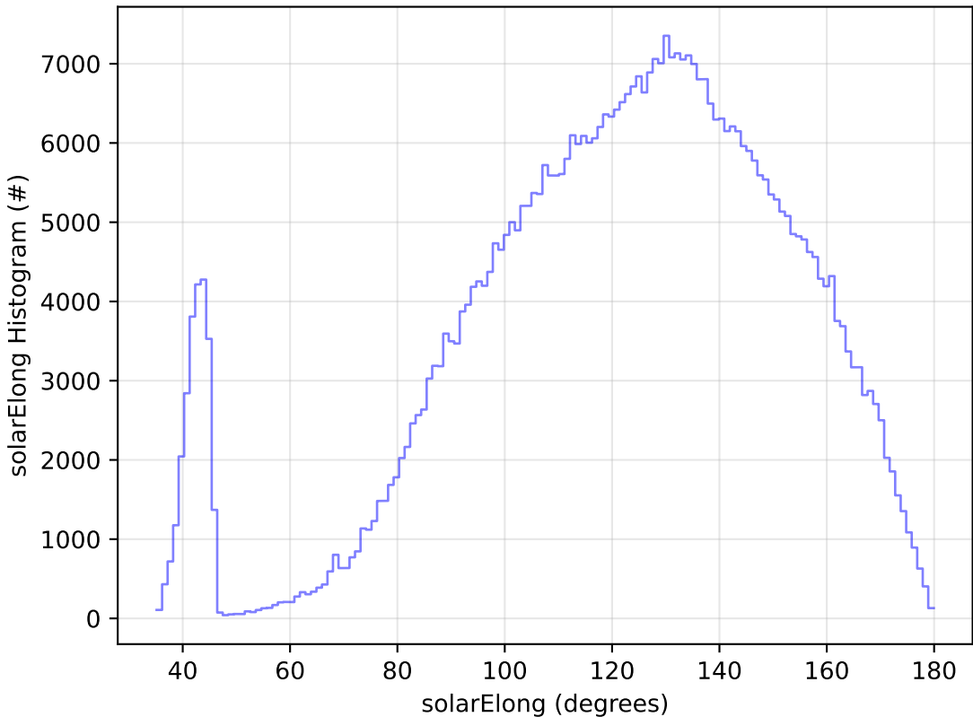
too_elab_r32_d3_griz_v3.4_10yrs All sky i band: solarElong Histogram
