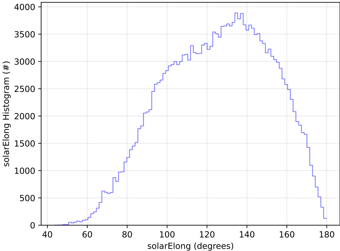
too_elab_r32_d3_griz_v3.4_10yrs All sky g band: solarElong Histogram
