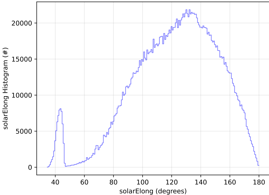
too_elab_r32_d3_griz_v3.4_10yrs All sky all bands: solarElong Histogram
