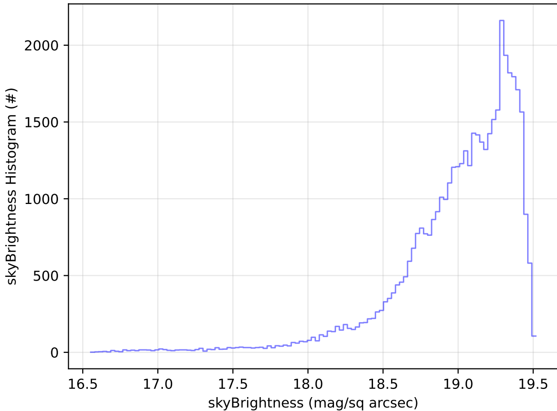
too_elab_r32_d3_griz_v3.4_10yrs Yr 1 z band: skyBrightness Histogram
