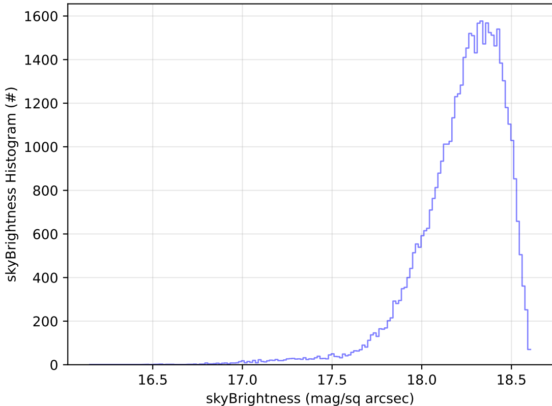
too_elab_r32_d3_griz_v3.4_10yrs Yr 1 y band: skyBrightness Histogram
