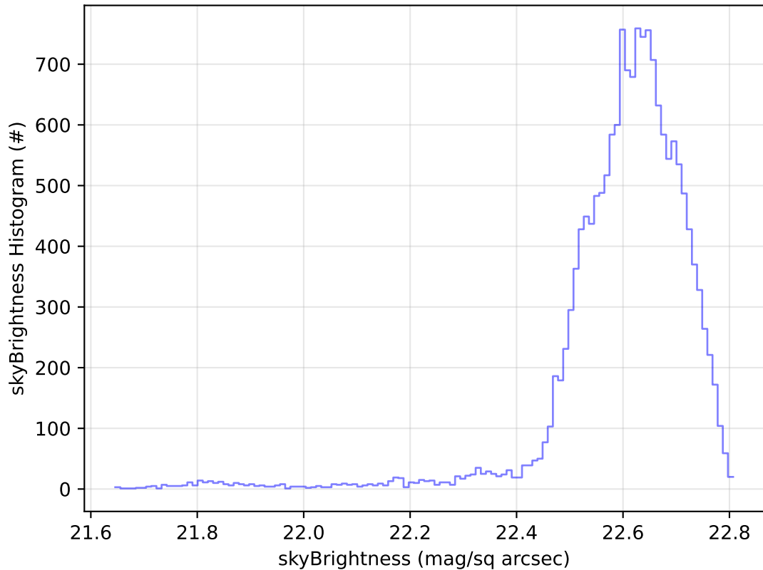
too_elab_r32_d3_griz_v3.4_10yrs Yr 1 u band: skyBrightness Histogram
