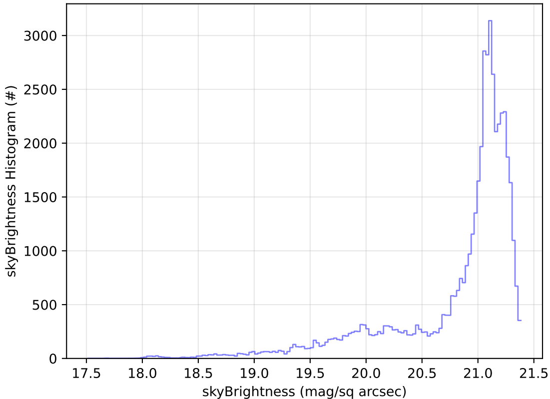
too_elab_r32_d3_griz_v3.4_10yrs Yr 1 r band: skyBrightness Histogram
