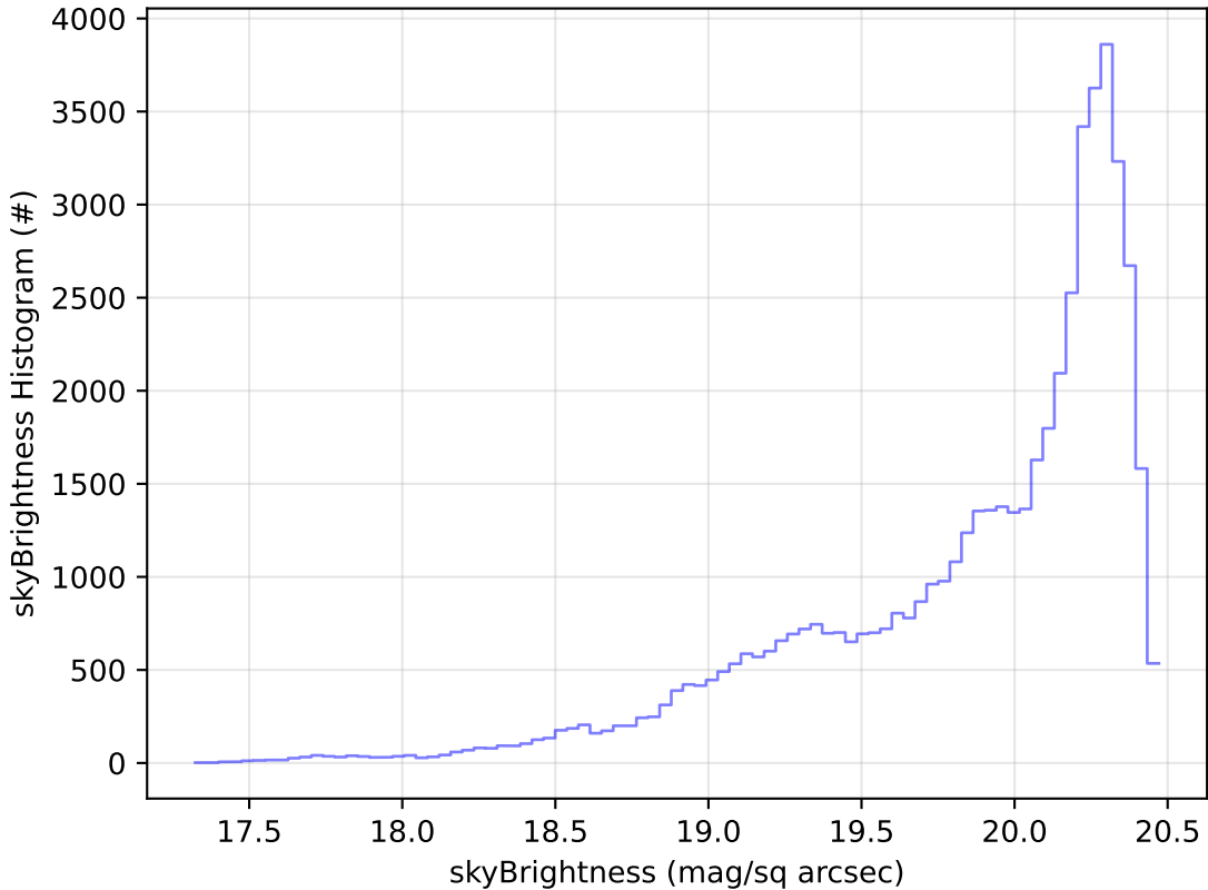
too_elab_r32_d3_griz_v3.4_10yrs Yr 1 i band: skyBrightness Histogram
