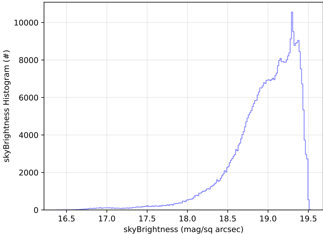
too_elab_r32_d3_griz_v3.4_10yrs WFD z band: skyBrightness Histogram
