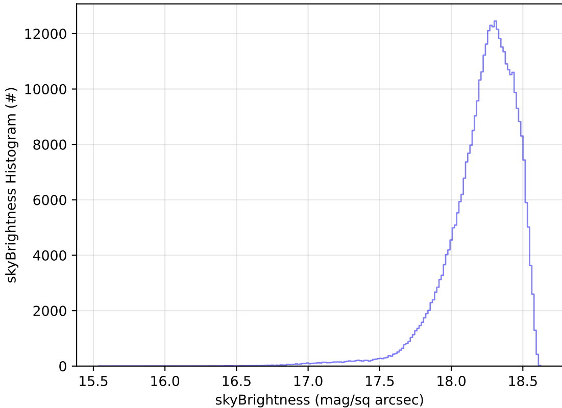
too_elab_r32_d3_griz_v3.4_10yrs WFD y band: skyBrightness Histogram
