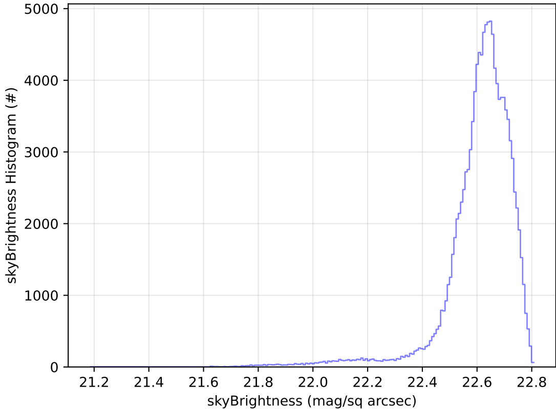
too_elab_r32_d3_griz_v3.4_10yrs WFD u band: skyBrightness Histogram
