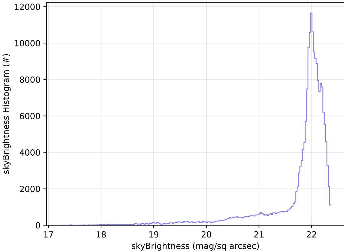
too_elab_r32_d3_griz_v3.4_10yrs WFD g band: skyBrightness Histogram
