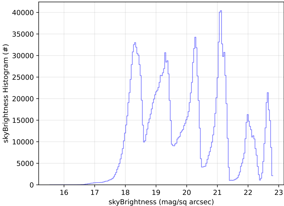
too_elab_r32_d3_griz_v3.4_10yrs WFD all bands: skyBrightness Histogram
