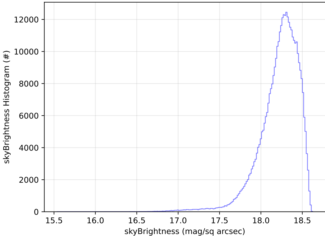
too_elab_r32_d3_griz_v3.4_10yrs All sky y band: skyBrightness Histogram
