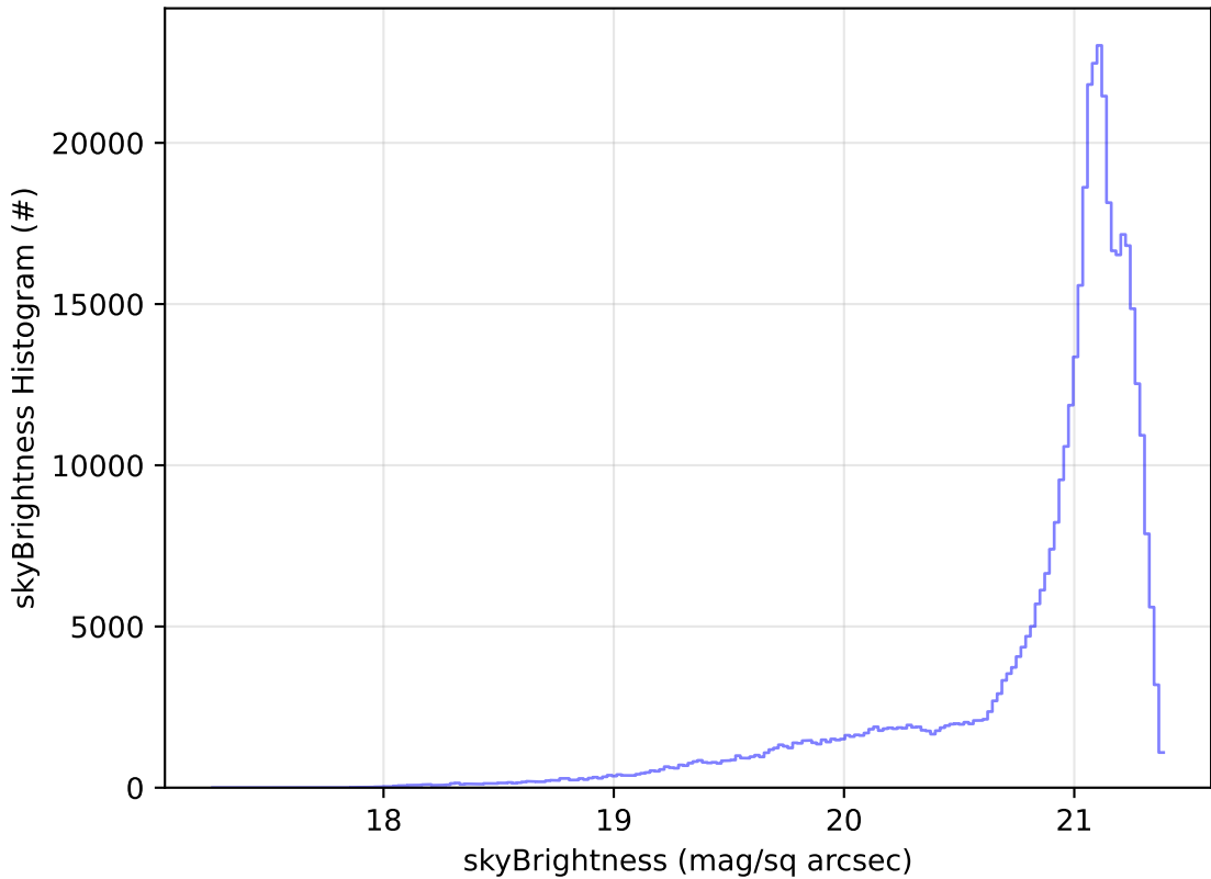
too_elab_r32_d3_griz_v3.4_10yrs All sky r band: skyBrightness Histogram
