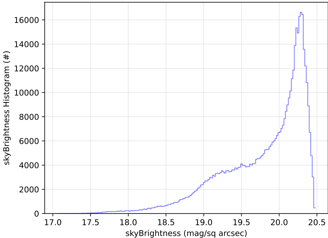
too_elab_r32_d3_griz_v3.4_10yrs All sky i band: skyBrightness Histogram
