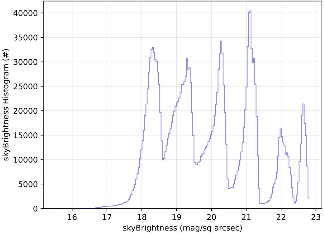
too_elab_r32_d3_griz_v3.4_10yrs All sky all bands: skyBrightness Histogram
