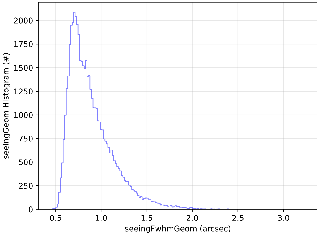
too_elab_r32_d3_griz_v3.4_10yrs Yr 1 r band: seeingGeom Histogram
