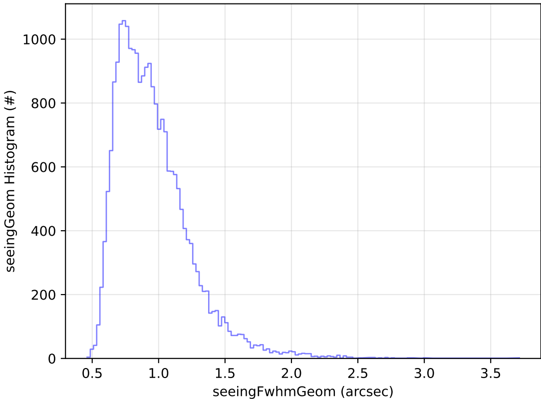
too_elab_r32_d3_griz_v3.4_10yrs Yr 1 g band: seeingGeom Histogram
