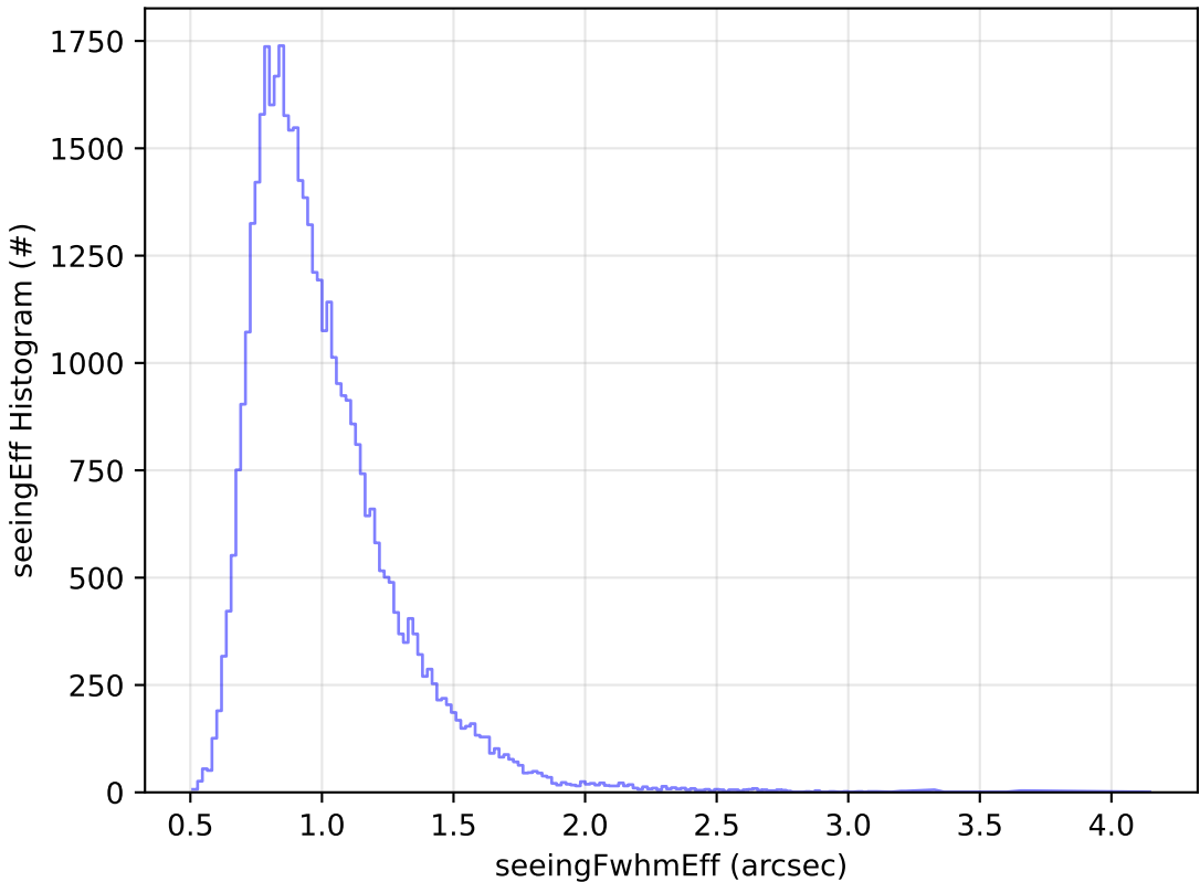
too_elab_r32_d3_griz_v3.4_10yrs Yr 1 z band: seeingEff Histogram
