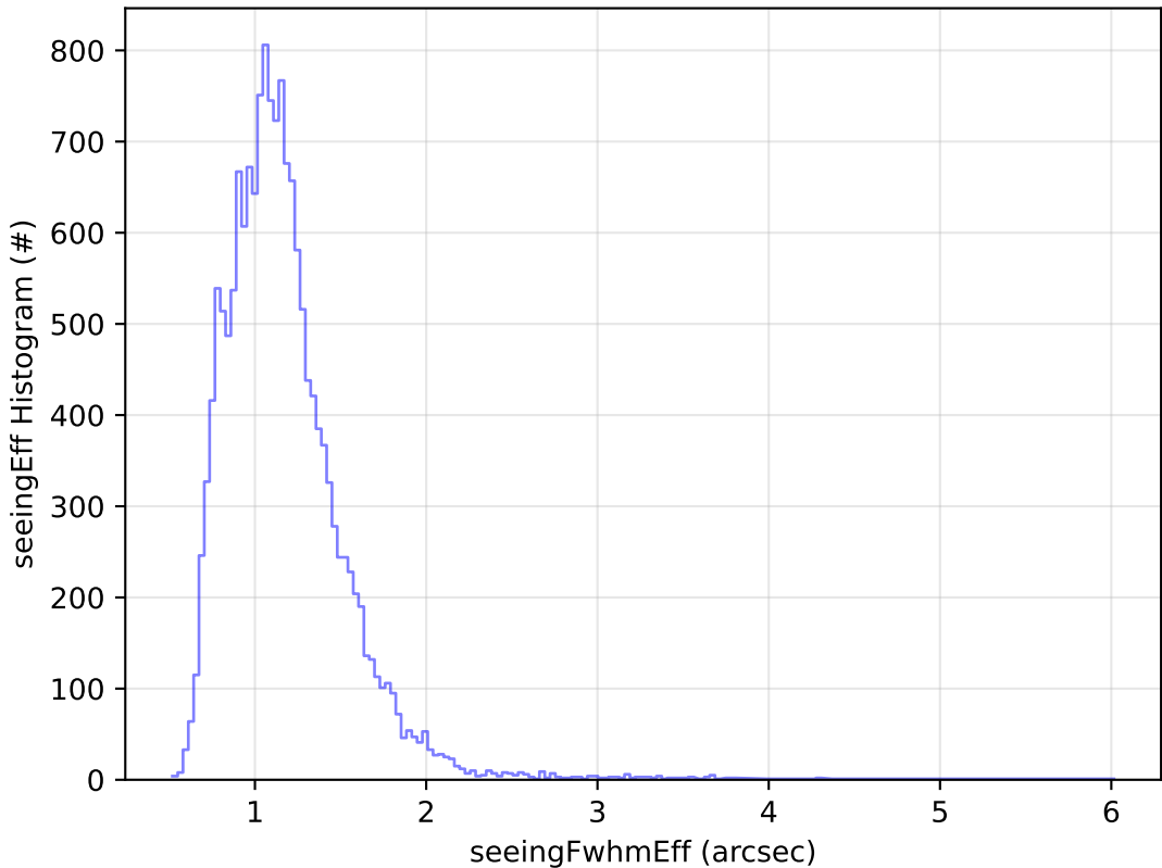
too_elab_r32_d3_griz_v3.4_10yrs Yr 1 u band: seeingEff Histogram
