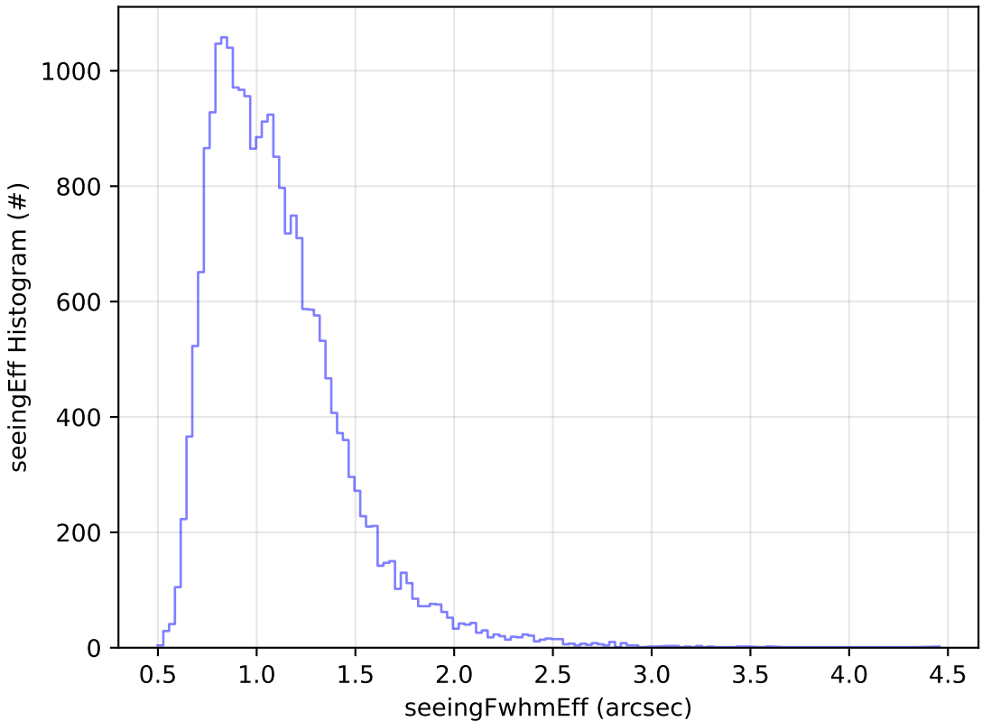
too_elab_r32_d3_griz_v3.4_10yrs Yr 1 g band: seeingEff Histogram
