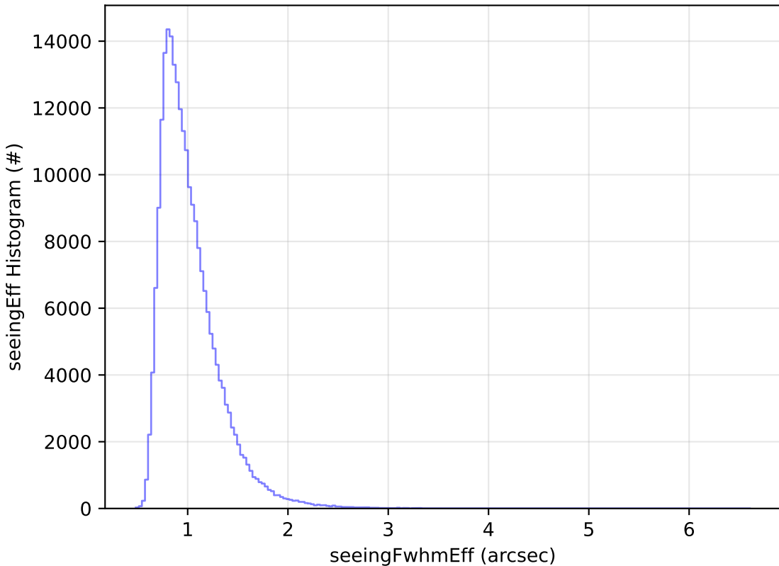
too_elab_r32_d3_griz_v3.4_10yrs Yr 1 all bands: seeingEff Histogram
