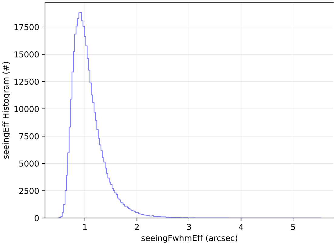
too_elab_r32_d3_griz_v3.4_10yrs WFD y band: seeingEff Histogram
