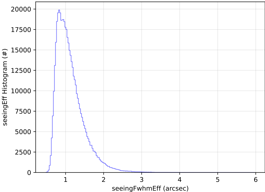
too_elab_r32_d3_griz_v3.4_10yrs WFD r band: seeingEff Histogram
