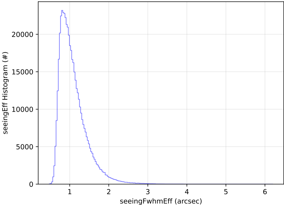
too_elab_r32_d3_griz_v3.4_10yrs WFD i band: seeingEff Histogram
