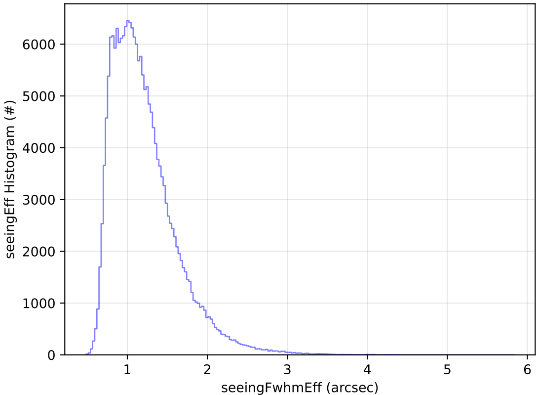
too_elab_r32_d3_griz_v3.4_10yrs WFD g band: seeingEff Histogram
