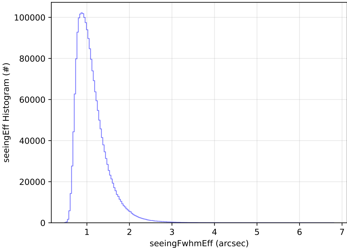
too_elab_r32_d3_griz_v3.4_10yrs WFD all bands: seeingEff Histogram
