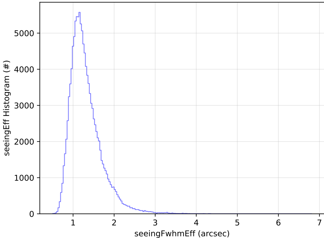
too_elab_r32_d3_griz_v3.4_10yrs All sky u band: seeingEff Histogram
