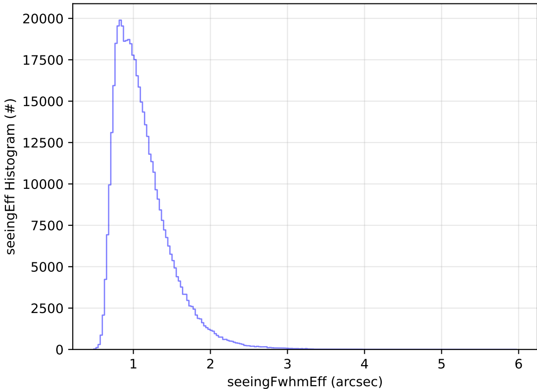
too_elab_r32_d3_griz_v3.4_10yrs All sky r band: seeingEff Histogram
