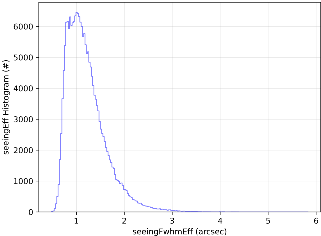
too_elab_r32_d3_griz_v3.4_10yrs All sky g band: seeingEff Histogram
