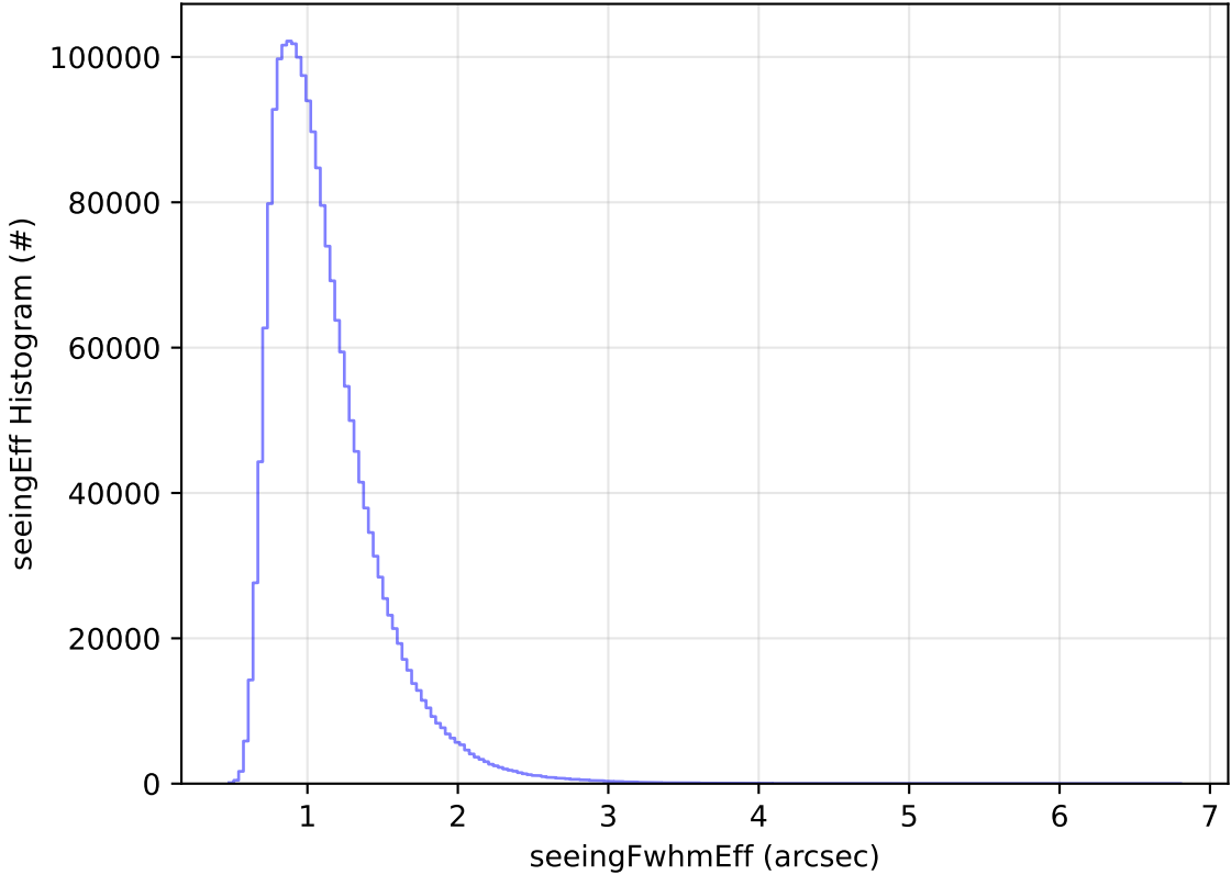
too_elab_r32_d3_griz_v3.4_10yrs All sky all bands: seeingEff Histogram
