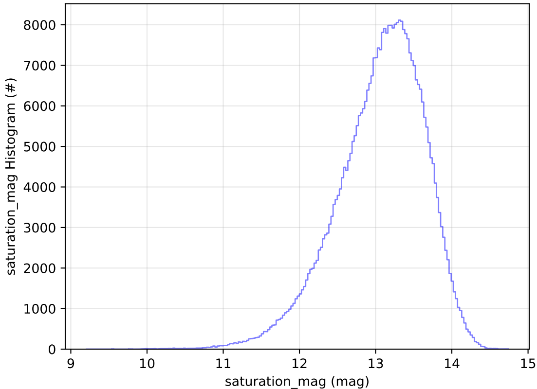
too_elab_r32_d3_griz_v3.4_10yrs WFD y band: saturation_mag Histogram
