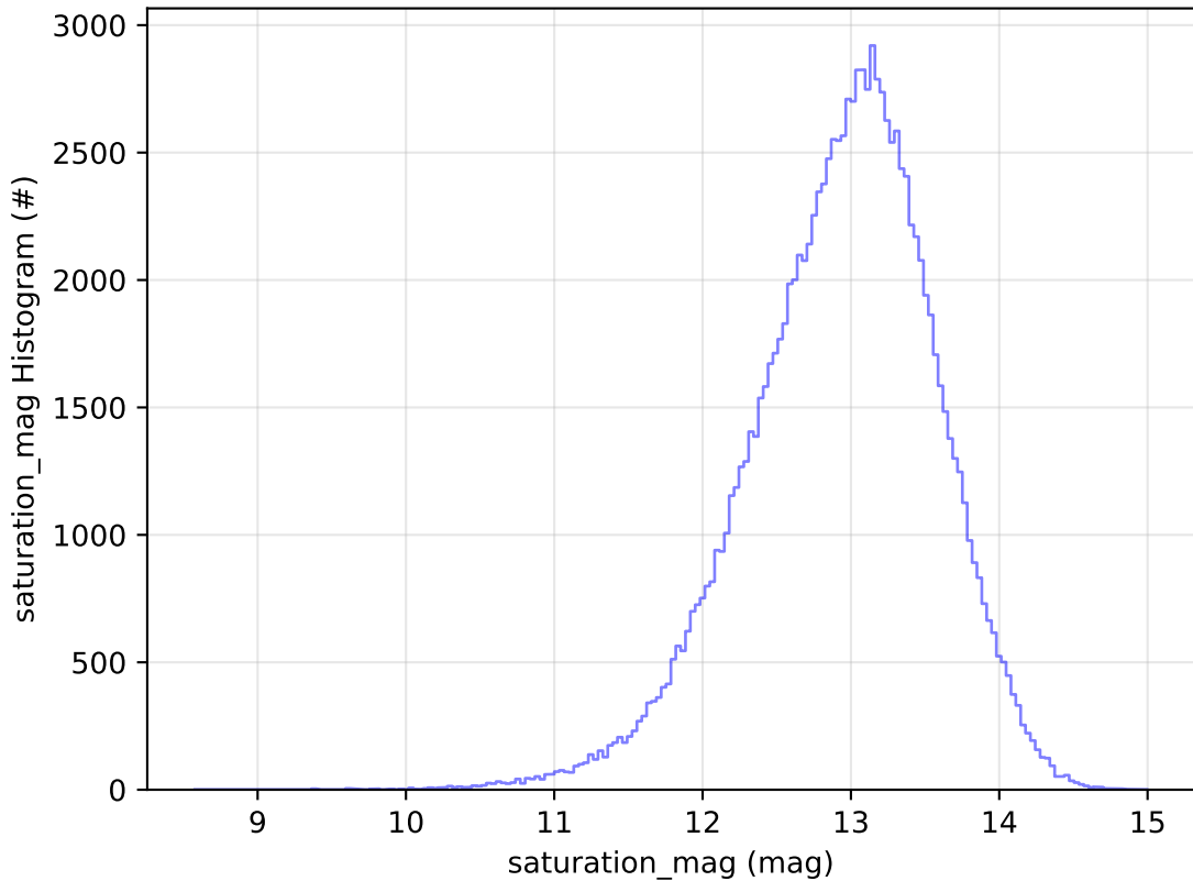
too_elab_r32_d3_griz_v3.4_10yrs WFD u band: saturation_mag Histogram
