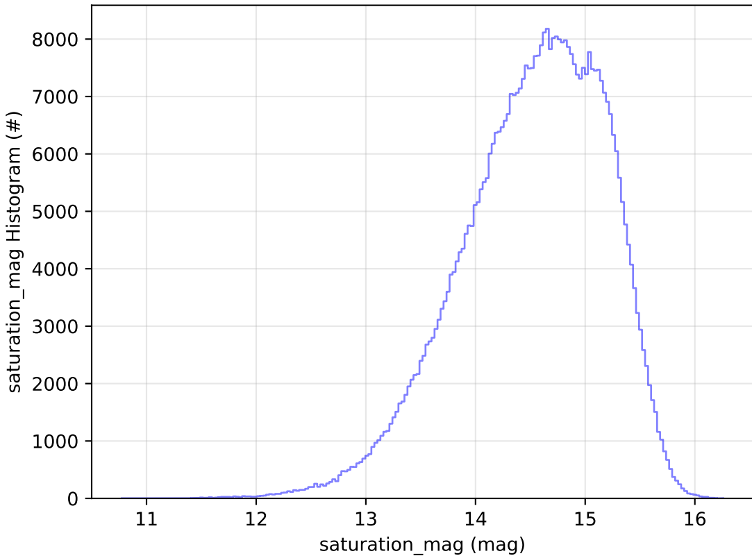
too_elab_r32_d3_griz_v3.4_10yrs WFD r band: saturation_mag Histogram
