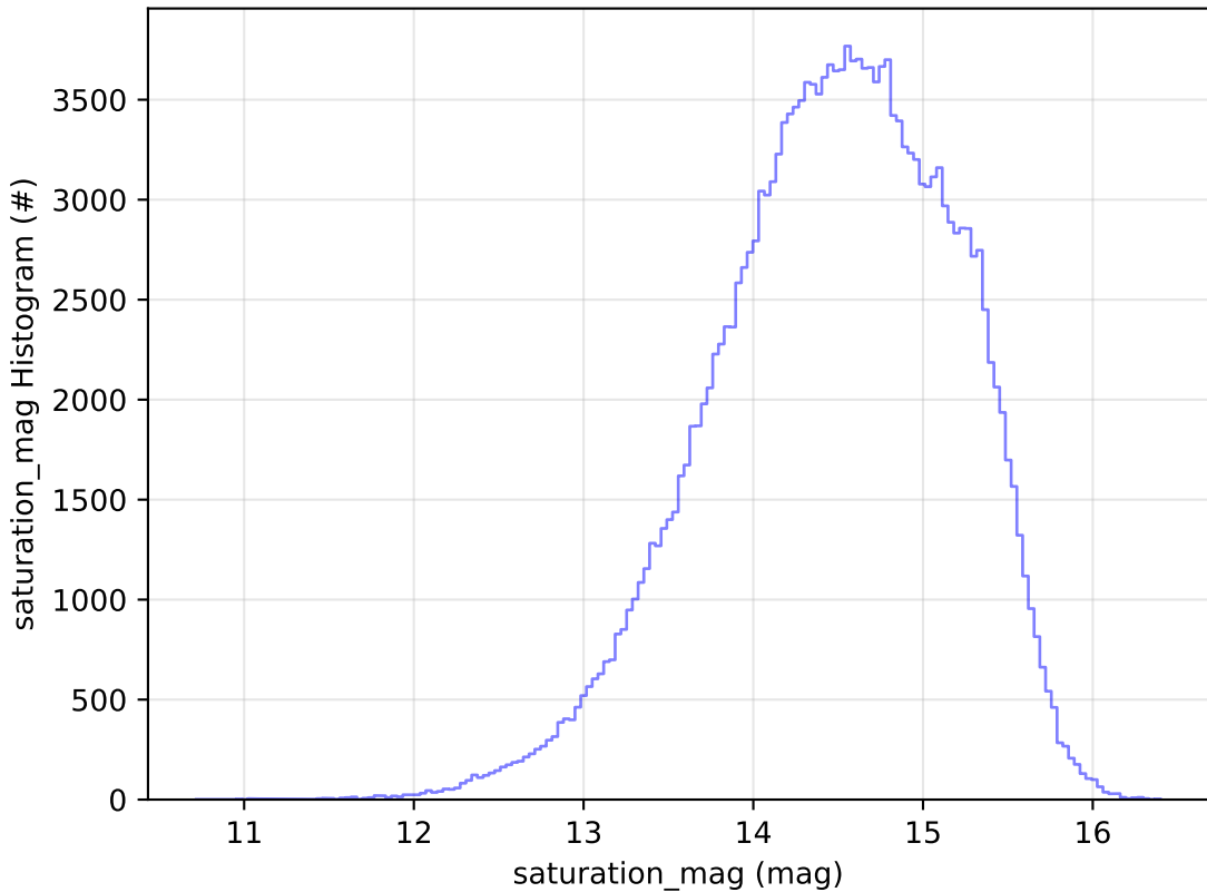
too_elab_r32_d3_griz_v3.4_10yrs WFD g band: saturation_mag Histogram
