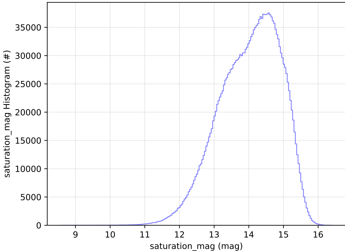
too_elab_r32_d3_griz_v3.4_10yrs WFD all bands: saturation_mag Histogram
