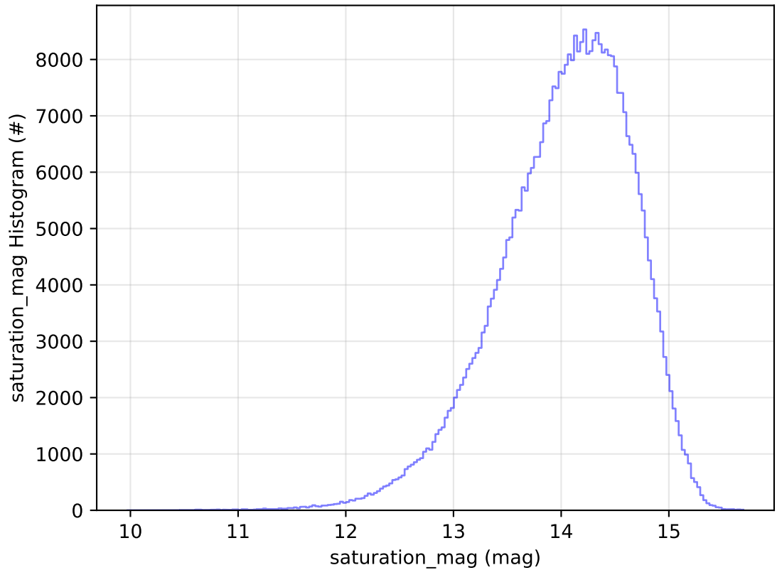
too_elab_r32_d3_griz_v3.4_10yrs All sky z band: saturation_mag Histogram
