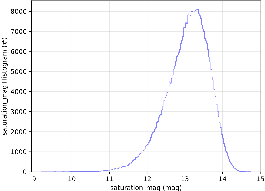
too_elab_r32_d3_griz_v3.4_10yrs All sky y band: saturation_mag Histogram
