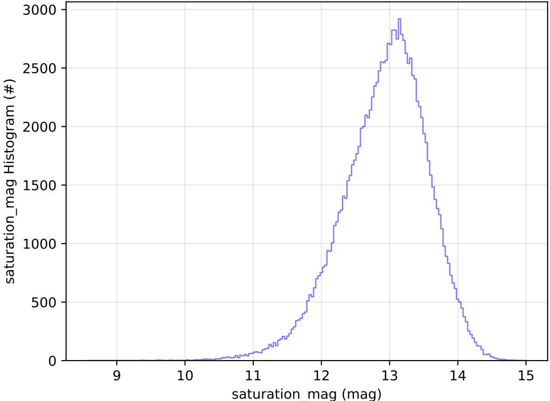
too_elab_r32_d3_griz_v3.4_10yrs All sky u band: saturation_mag Histogram
