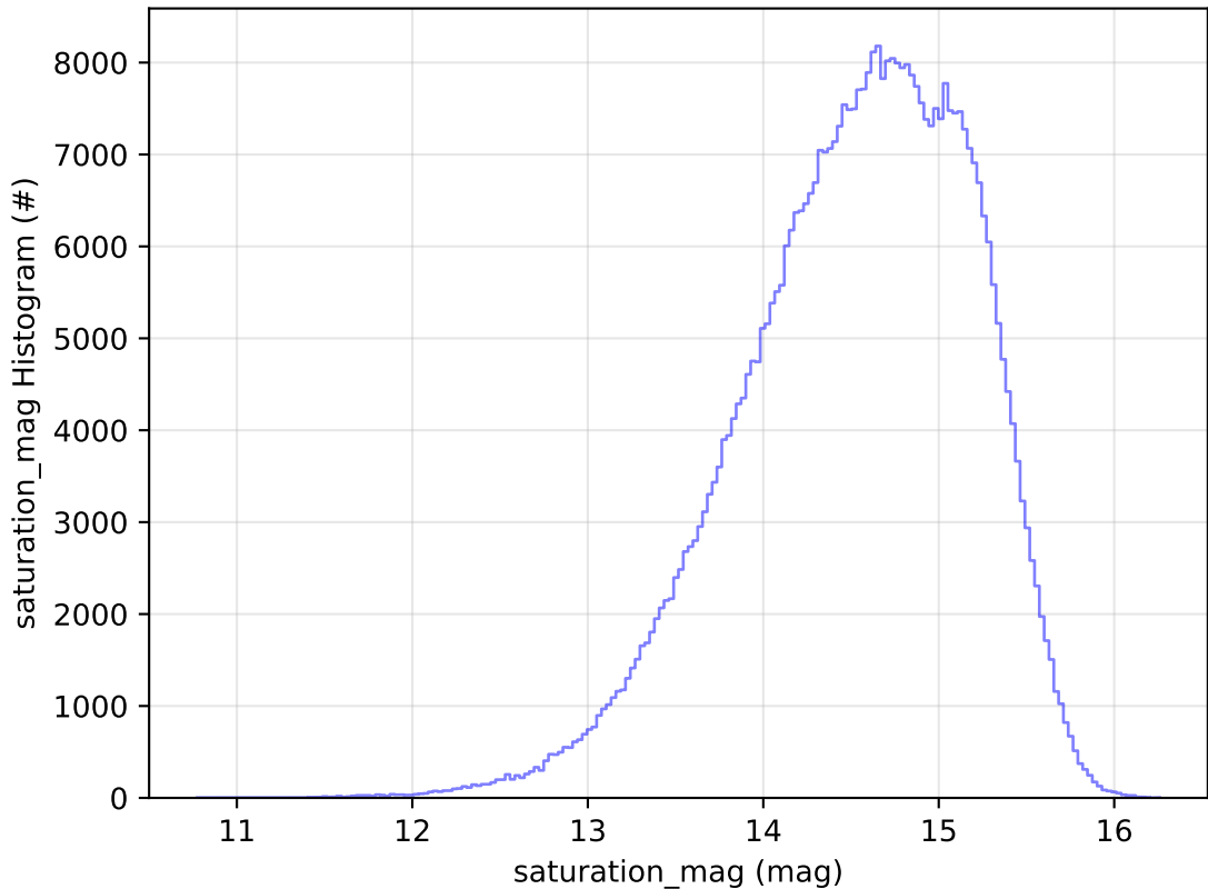
too_elab_r32_d3_griz_v3.4_10yrs All sky r band: saturation_mag Histogram
