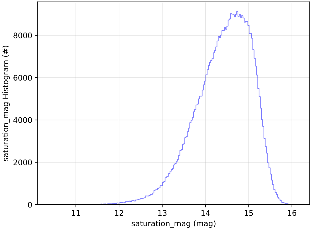
too_elab_r32_d3_griz_v3.4_10yrs All sky i band: saturation_mag Histogram
